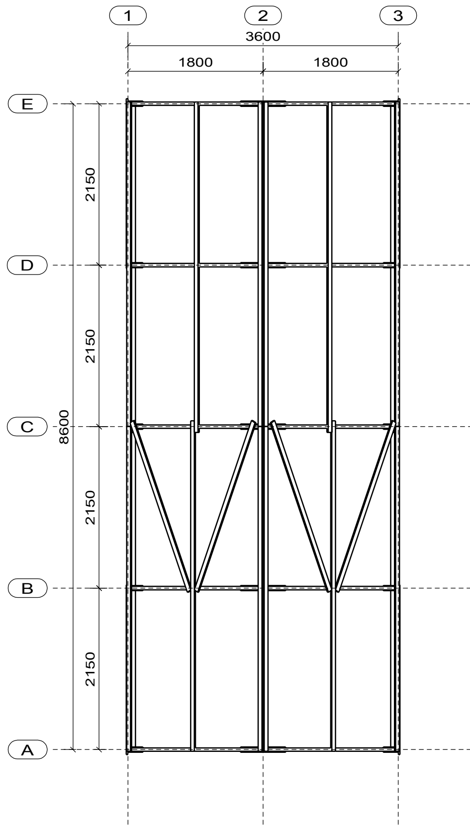
PLAN
